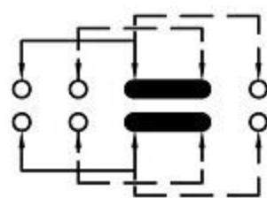
SCHMATIC (SHORTING)
